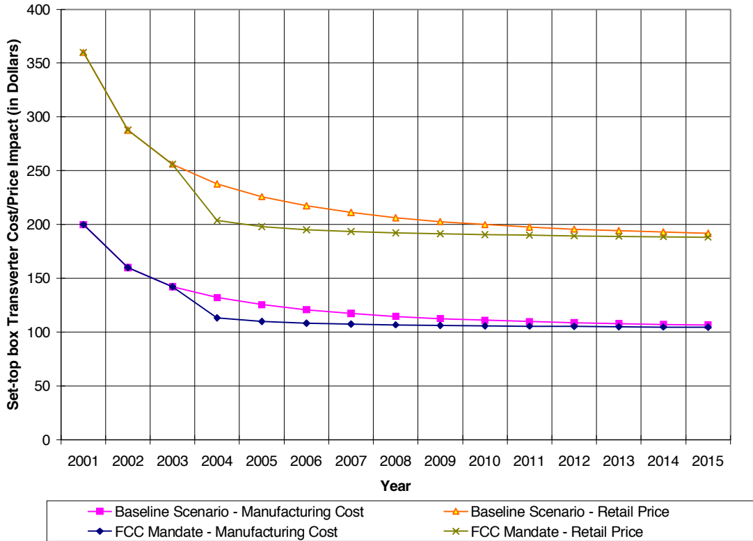
Figure 1-4 SDTV Set-top Box Transverter Cost/Price Analysis
