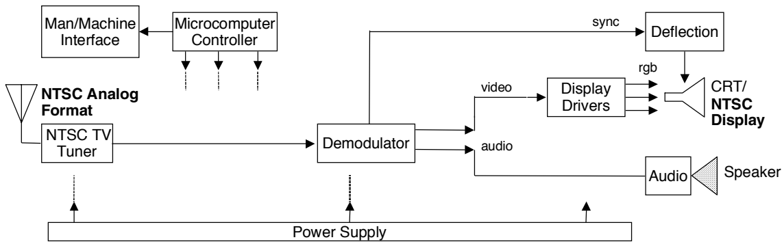
Figure 3-2 Simplified Block Diagram of Leader Model NTSC Analog TV Receiver
